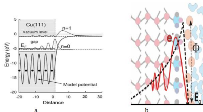
Figure (2-12): Schematic illustration of (a) model potential of electron transfer at band probability at the Cu /liquid[8], and (b) tunneling process[9].
