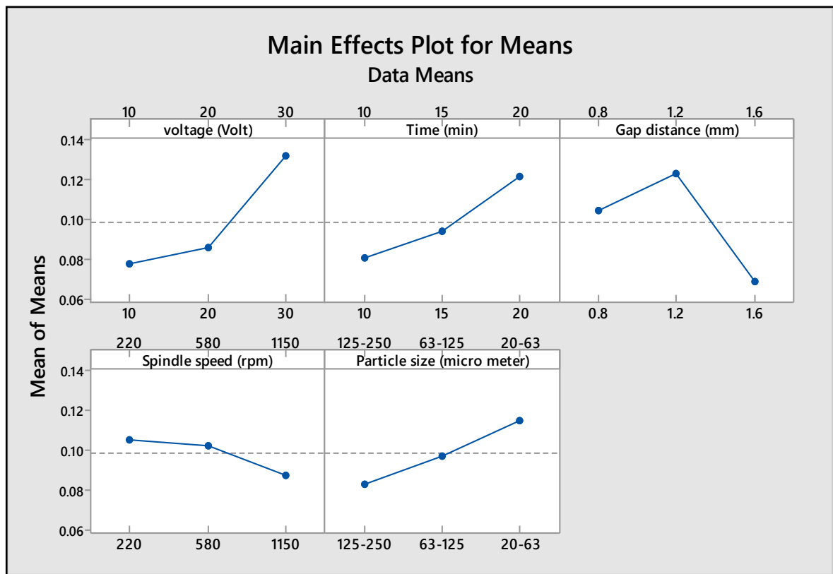
Figure 3: Means of Microhardness
