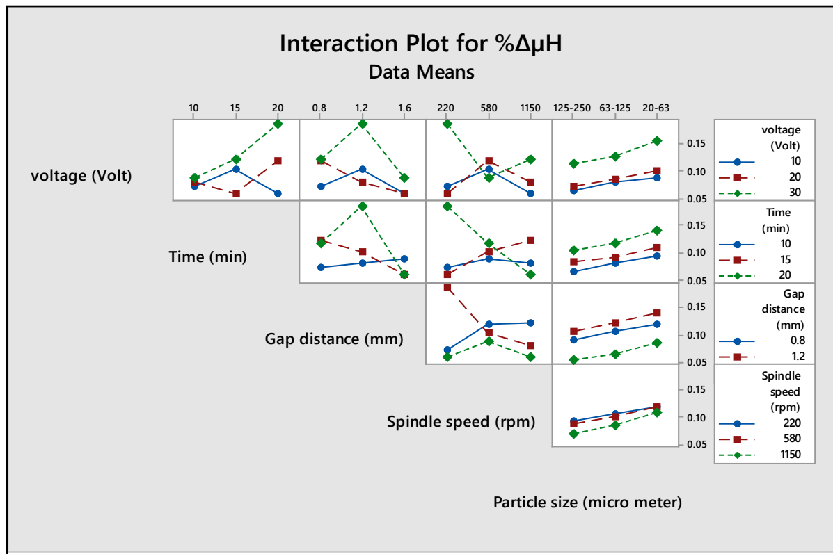
Figure 4: Interaction plot for % \Delta MH
