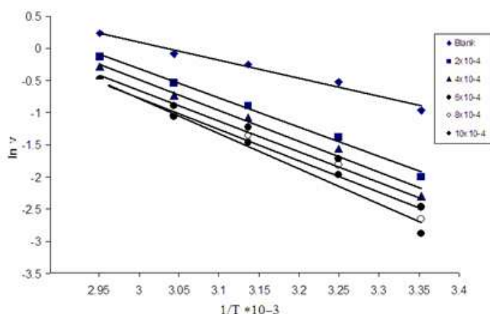
Fig.7: Plots of \ln(\text{corrosion rate}) versus 1/T \times 10^{-3} for different Concentration.
