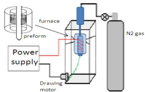
Fig. 1 Schematic diagram of apparatus perform
