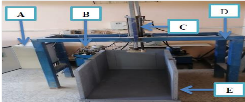
Figure 3: Device for vibratory impact: A. Data acquisition, B. Electro-hydraulic apparatus, C. Shaft encoder, D. Steel frame loading, and E. Steel container
