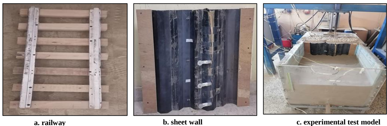
Figure 2: Laboratory models; a. the rail track, b. the steel sheet wall, and c. experimental test model with sandy soil.
