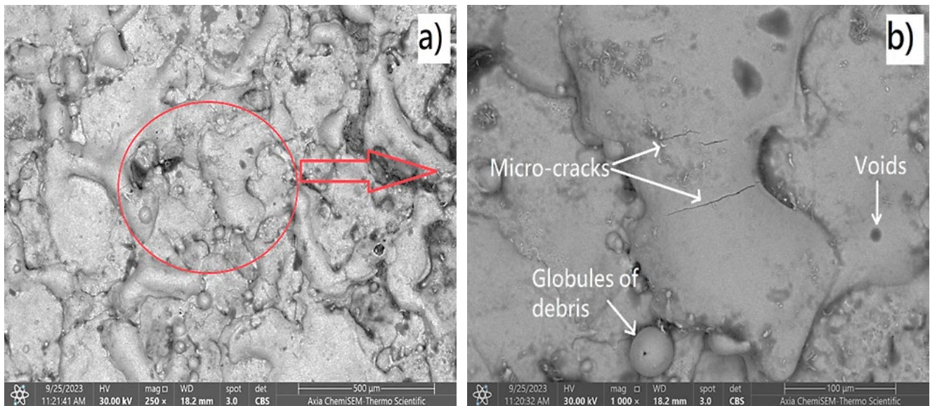
Figure 7: Micrographs of machined surface using 4 g/l of added nano- \text{Al}_2\text{O}_3 , a) with 250x magnification b) with 1000x magnification
