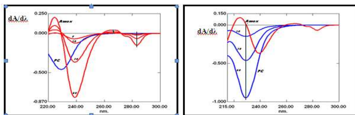
Fig (2): a- ^1D spectra for 5–60 \mu\text{g.mL}^{-1} Amox and 30 \mu\text{g.mL}^{-1} PC at 267 and 283.5 nm, b- ^1D spectra for 10–60 \mu\text{g.mL}^{-1} PC and 30 \mu\text{g.mL}^{-1} Amox (zero crossing) at 229 nm.
