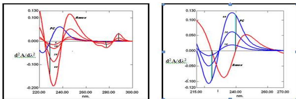
Fig (3): ^2D spectra for 5–60 \mu\text{g.mL}^{-1} Amox and 30 \mu\text{g.mL}^{-1} PC at 288, 277.5 and 229 nm. b-
