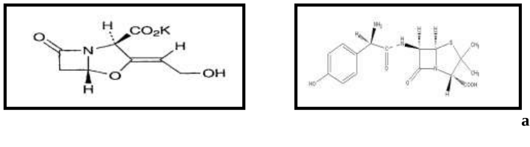
Fig (1): Structure of a- potassium clavulanate, b- Amoxicillin trihydrate
