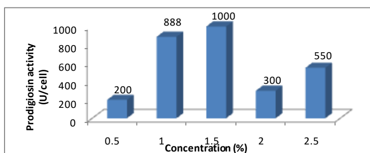
Fig (4): Effect of casein hydrolysate concentration on prodigiosin production by S. marcescens S11 after incubation in shaker incubator (150 rpm) for 24hrs at 28°C
