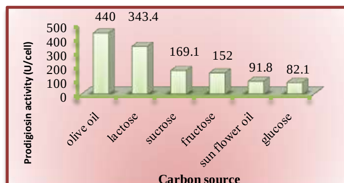
Fig (1): Effect of carbon source on prodigiosin production by S. marcescens S11 after incubation in shaker incubator (150 rpm) for 24hrs at 28°C.
