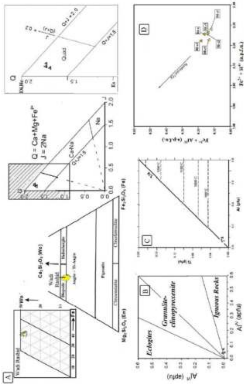
Fig. 4 : A: Plot of clinopyroxene compositions of Wadi Rashid in the En—Wo—Fs ( \text{Mg}_2\text{Si}_2\text{O}_6 — \text{Ca}_2\text{Si}_2\text{O}_6 — \text{Fe}_2\text{Si}_2\text{O}_6 ) diagram with the nomenclature fields of Morimoto et al. , (1988). B : \text{Al}^{\text{IV}} vs. \text{Al}^{\text{VI}} diagram of Aoki and Shiba (1973) shows that the crystallization pressure of WR clinopyroxenes is low and they plot within “igneous clinopyroxene” field. C: A plot of Ti vs Al concentrations (Yagi and Onuma 1967, Sepp and Kanzmann 2001), illustrate that the crystallization temperature of WR clinopyroxenes is slightly below 900 °C, D: \text{Fe}^{2+} + \text{Si}^{4+} – \text{Fe}^{3+} + \text{Al}^{\text{IV}} relationships for WR clinopyroxenes, showing the negligible increasing f\text{O}_2 during the agpaaitic processe. Data from Table 1; a.p.f.u. = atoms per formula unit.
