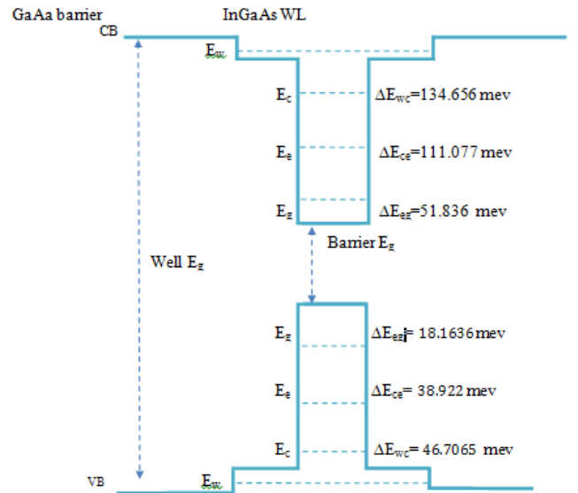
Figure 2: energy difference diagram in present simulation
