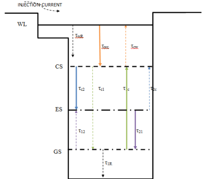
Figure 1: Energy band diagram of the QD-based SOA and the main processes.
