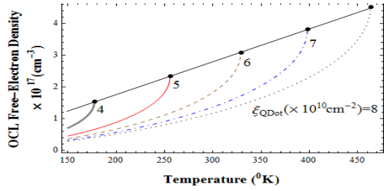
Fig. 6. OCL free-electron density, \bar{f}_{\text{OCL}}^e vs. temperature, T for different values of surface density of QDs; \xi_{\text{QDot}} (\times 10^{10} \text{ cm}^{-2}) = 4, 5, 6, 7 and 8 . The straight line marks the QD micro-cavity maximum operating temperature.
