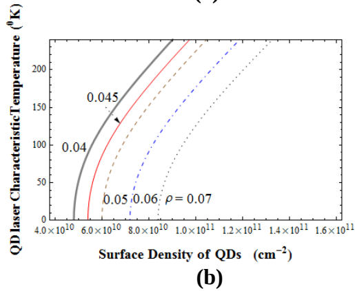
Fig. 5. Laser Characteristic Temperature, T_0 vs. Surface Density of QDs processes for; (a) Constant component of internal loss; k_0 (\text{cm}^{-1}) = 0, 1, 3, 6 and 10 respectively, (b) RMS of relative QD-size fluctuations; \rho = 0.04, 0.045, 0.05, 0.06 and 0.07 respectively, (c) Mean size of QDs; M_{QDot} (\text{\AA}) = 120, 135, 150, 180 and 200 respectively, and (d) Optical confinement factor in the QD layer; \Gamma = 0.04, 0.05, 0.06, 0.07 and 0.08 .
