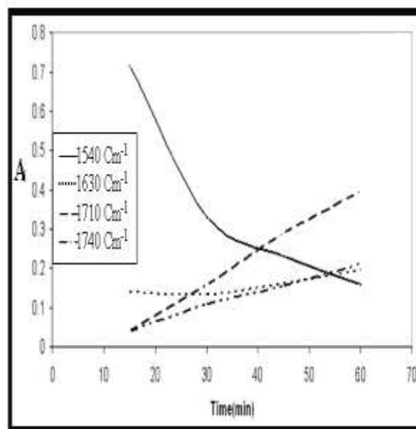
Fig (12): Dependence of the peaks for PVC films stabilized with Co stearate on the time of thermal degradation at 195 °C in air [ A_i = \log (T1800 / T_i) ]
