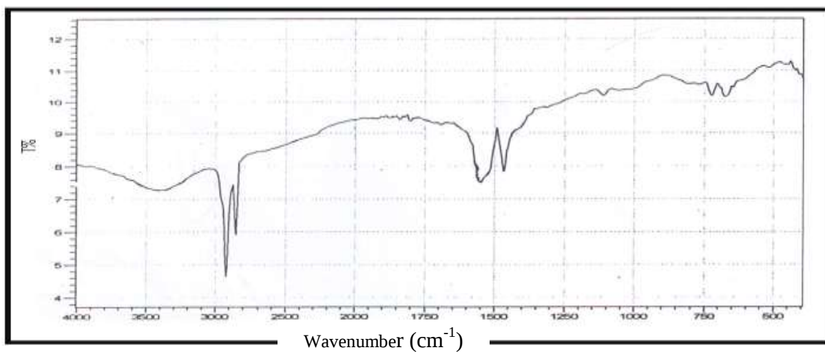
Fig (3): Infrared spectrum for Co stearate
