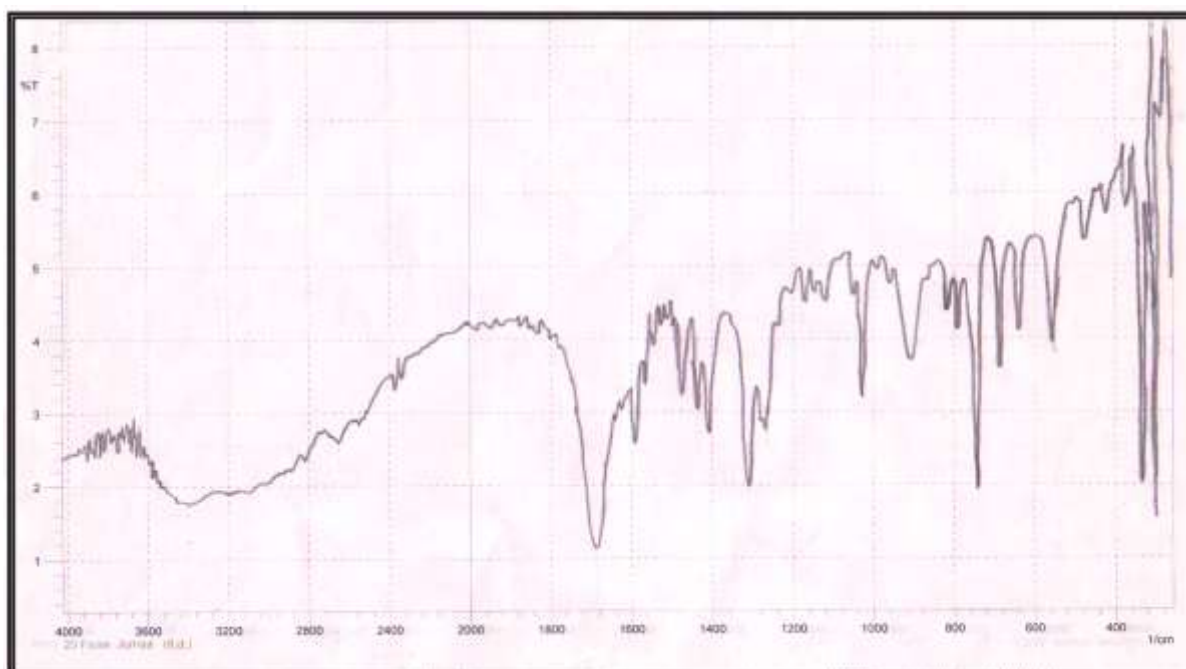
Fig (1): Infrared spectrum for stearic acid
