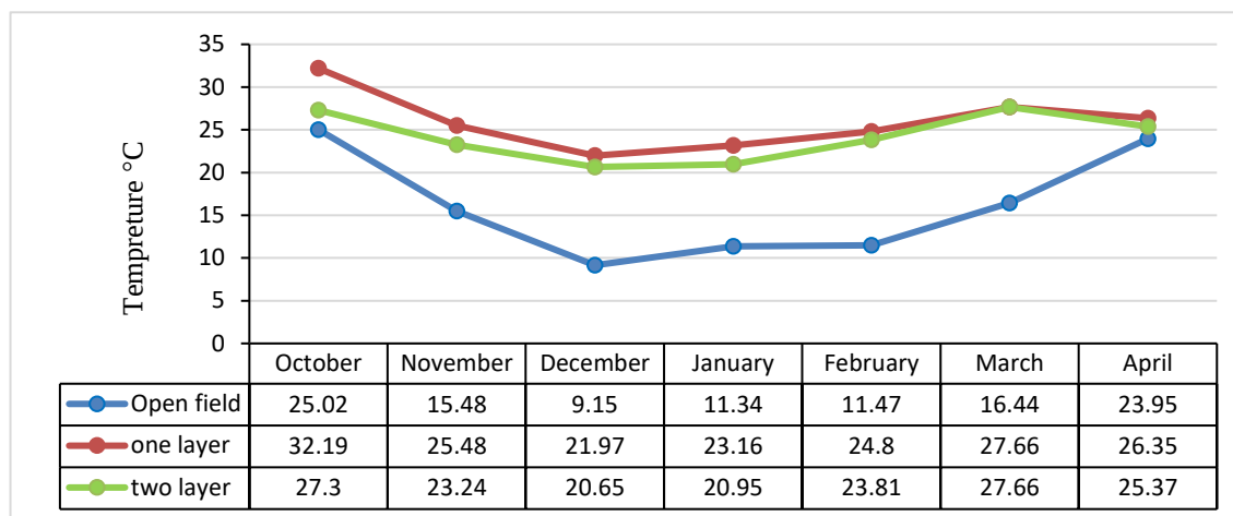
Figure (1): Average monthly temperature (°C) during the day hours at the location of the experiment
