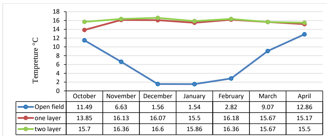
Figure (2): Average monthly temperature (°C) during the night hours at the location of the experiment
