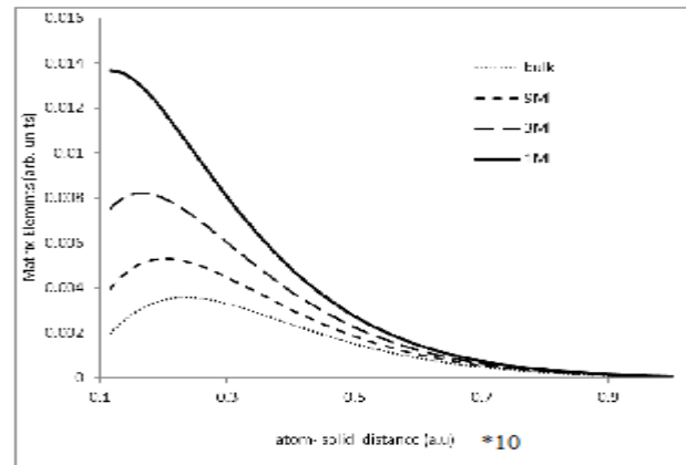
Fig.1: Matrix elements for H^- - ion in front of Al (111) thin films using the Perturbative method.
