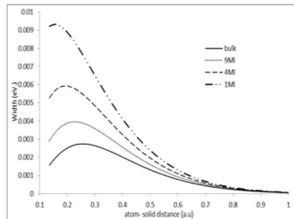
Fig.2: Total transition rates for H^- / Al (111) thin films using the Perturbative method
