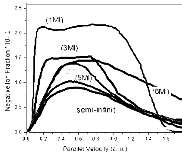
Fig.3: Negative ion fraction for H^- / Al (111) thin films using the Perturbative
