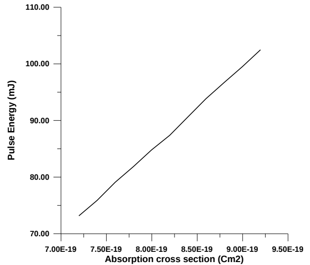
Fig.(2): The behavior of pulse energy as function of the ground state absorption cross section of saturable absorber
