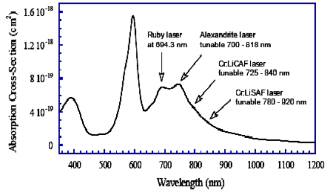
Figure 1: Cr : YSO absorption spectrum [10]
