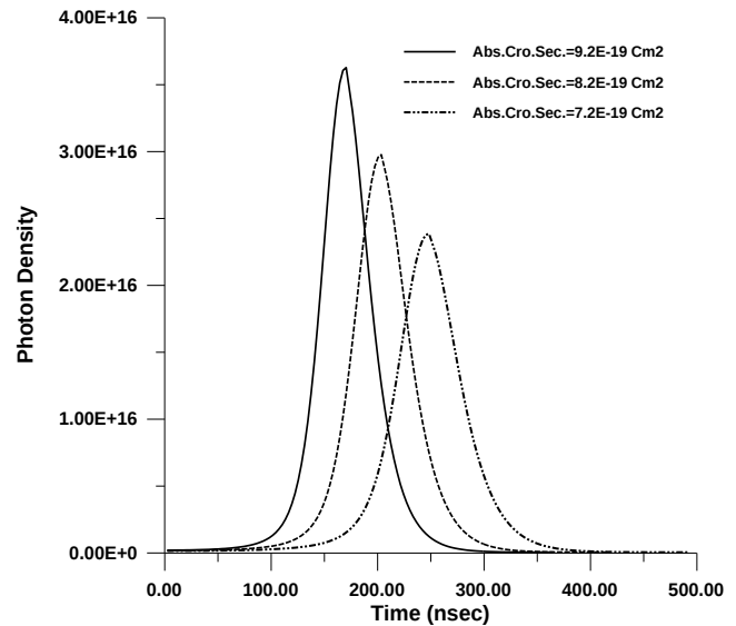
Fig.(6): profiles of pulse as function of the ground state absorption cross section of saturable absorber
