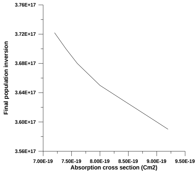
Fig.(4): The behavior of final population inversion as function of the ground state absorption cross section of saturable absorber
