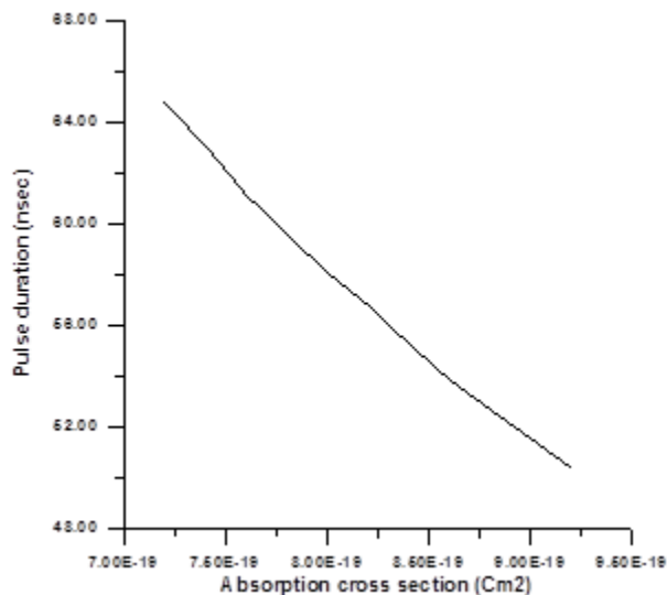
Fig.(5): The behavior of pulse duration as function of the ground state absorption cross section of saturable absorber
