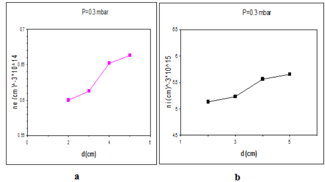
Fig.(6): The relation between (a) electron density, (b) ion density, as a function to the distance.
