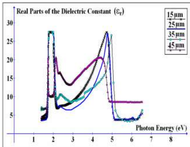
Fig. (5) Real part of Dielectric Constant of (PVA- \text{CoCl}_2 ) for different thickness films.
