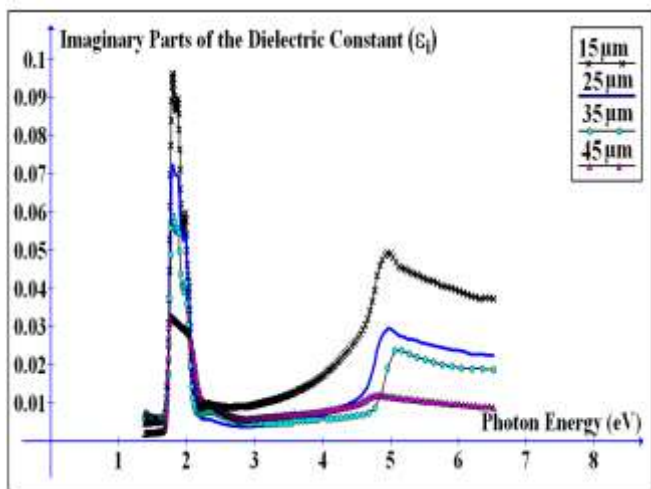
Fig. (6) Imaginary Part of Dielectric Constant of (PVA- \text{CoCl}_2 ) for different thickness films.
