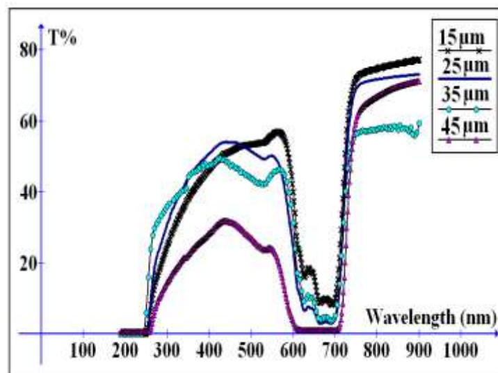
Fig. (1) Transmission Spectra of (PVA- \text{CoCl}_2 ) different thickness films.
