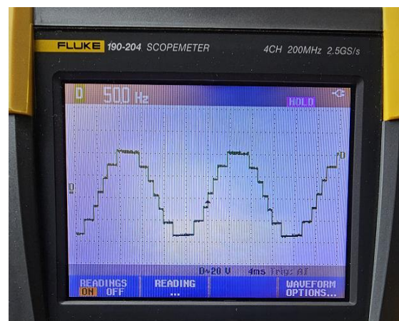
(b) Experimental Output voltage waveform
