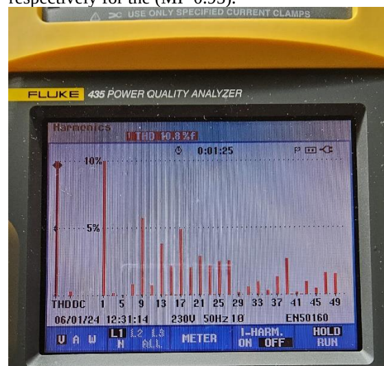
(a) Experimental FFT Analysis
