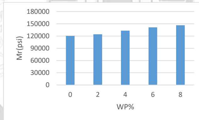
Fig.9 Impact of WP% on resilient modulus
