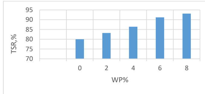
Fig.8 Impact of WP % on TSR.
