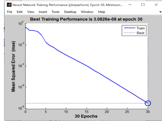
Fig. (3): Neural network training performance at 30 epochs.
