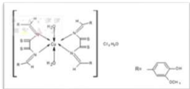
Fig.15 Proposed structure of the complex \text{CuLH}_3
