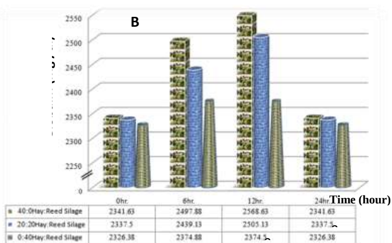
Fig(3): The main effect of IP (A) and AH: RS (B) on the pattern of BGC during 0, 6, 12 and 24 hrs. post morning feeding.
