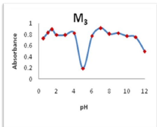
Fig.-7: pH-Absorbance curve for dye M 3
