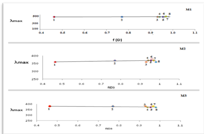
Fig.- 11: \lambda_{max} With f(D) for (M1- M3) : Where ; 1=1,4-dioxane, 2= ethyl acetate, 3= acetone, 4= methanol, 5= ethanol, 6 = DMF, 7=DMS, 8= water
