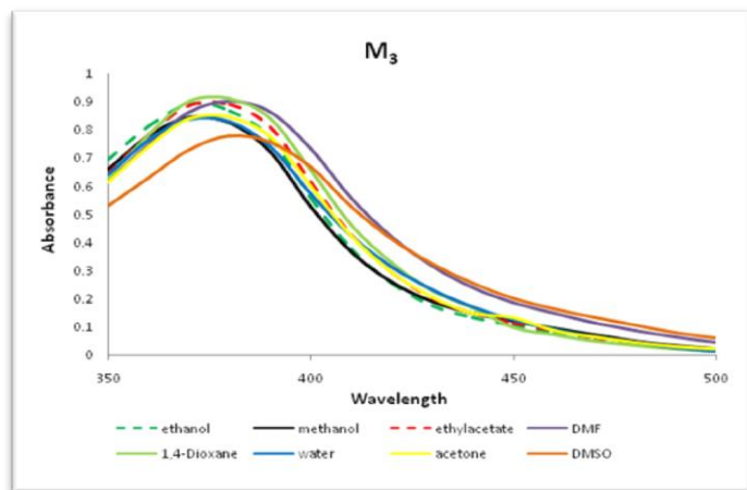
Fig.- 10: Absorption spectra of dye (M3) in various solvents
