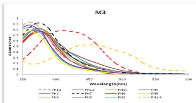
Fig.- 4: The electronic spectra of M3 at different pH values .
