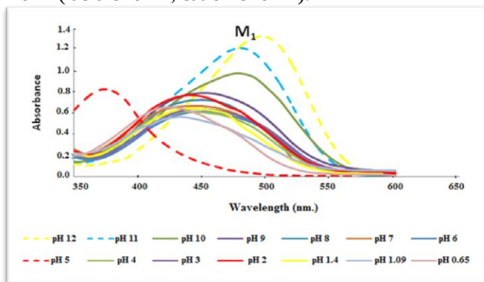
Fig.- 2: The electronic spectra of M1 at different pH values
