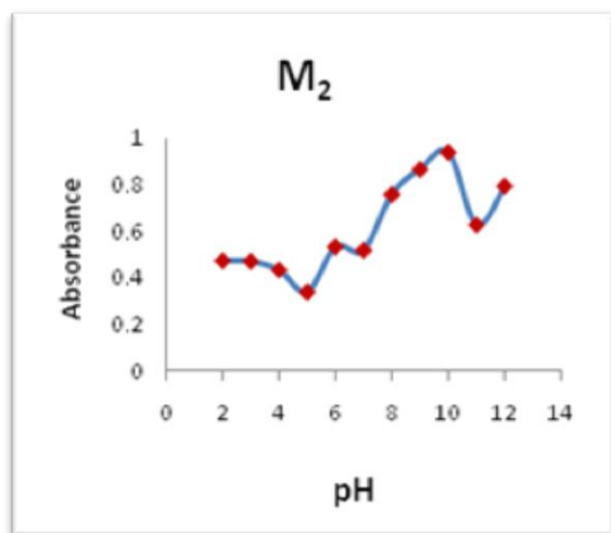
Fig.-6: pH – Absorbance curve for dye M 2
