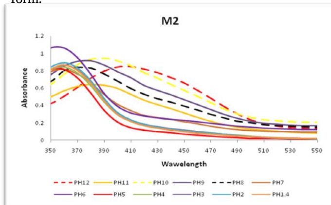
Fig.- 3 : The electronic spectra of M2 at different pH values
