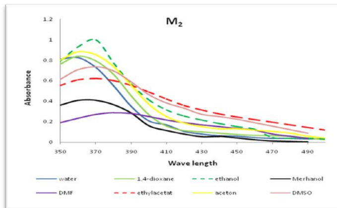
Fig.-9: Absorption spectra of dye (M 2 ) in various solvents
