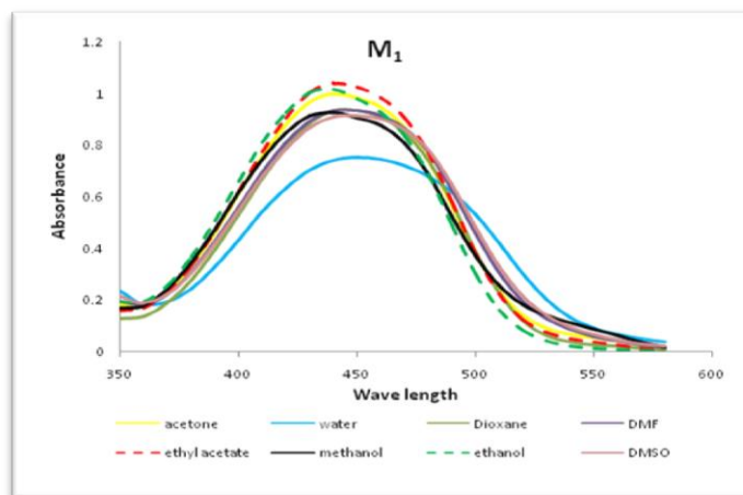
Fig.- 8: Absorption spectra of dye (M 1 ) in various solvents
