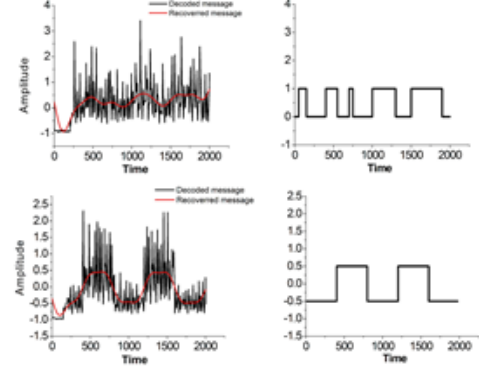
Fig. 8: Chaotic communication based on CSK. Transmitter signals in the left column and receiver signals in the right column. (a) Chaotic oscillation in the transmitter and receiver with a random message. (b)
