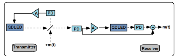
Fig. 7: Schematic diagrams of scheme for chaos synchronization and communications using QD-LEDs with OPEFB. Chaos shift keying (CSK) system.
