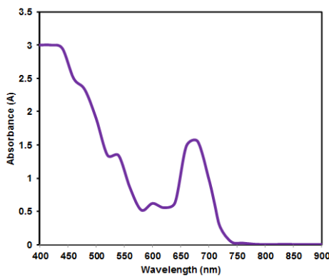
Fig. 2. The absorbance spectrum of pepper oil.
