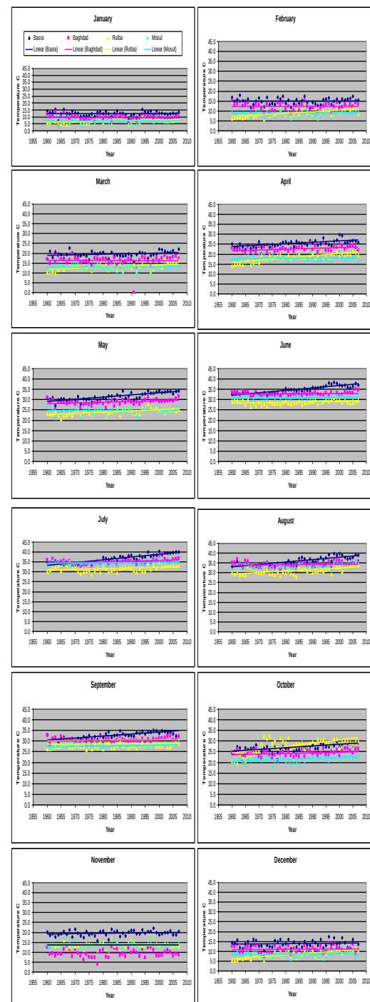
Figure 2: Average monthly temperature of Basra, Baghdad, Mousul and Rutba since 1960 till 2007.
