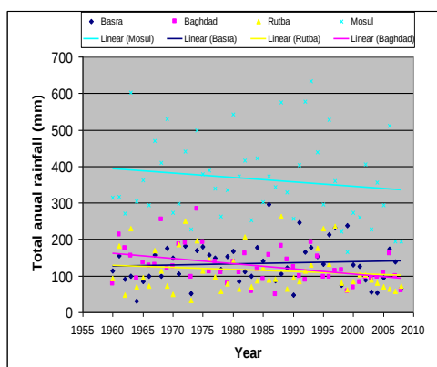
Figure.3: Annual rainfall average of Mosul, Baghdad, Basra and Rutba since 1960 till 2008.
