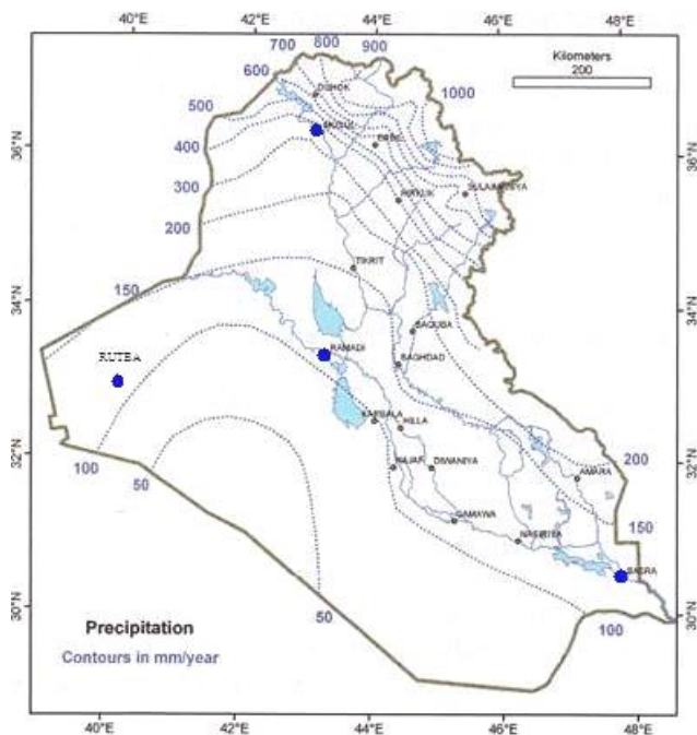
Figure.1: Precipitation map (After Alsam et al.1990 in Jassim and Goff, 2006) displaying the meteorological station as a solid circles.
