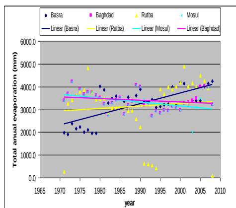
Figure.4: Evaporation average of Mosul, Baghdad, Basra and Rutba since 1970 till 2008.
