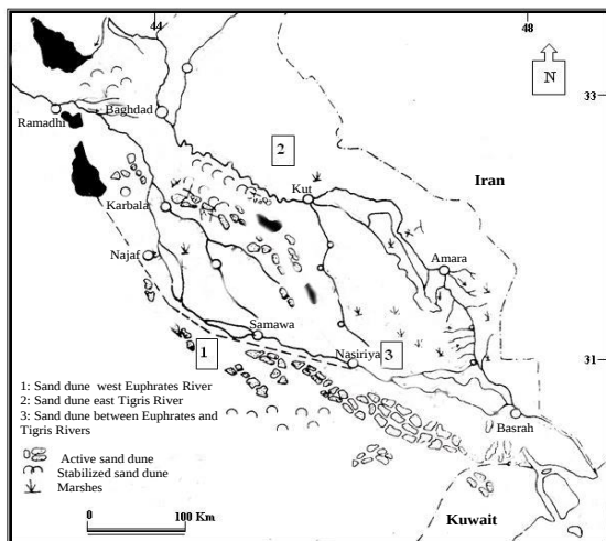
Fig-2: Distribution of sand dunes in Iraq and NW Arabian gulf (modified after Al-Rayhani, 1986)
