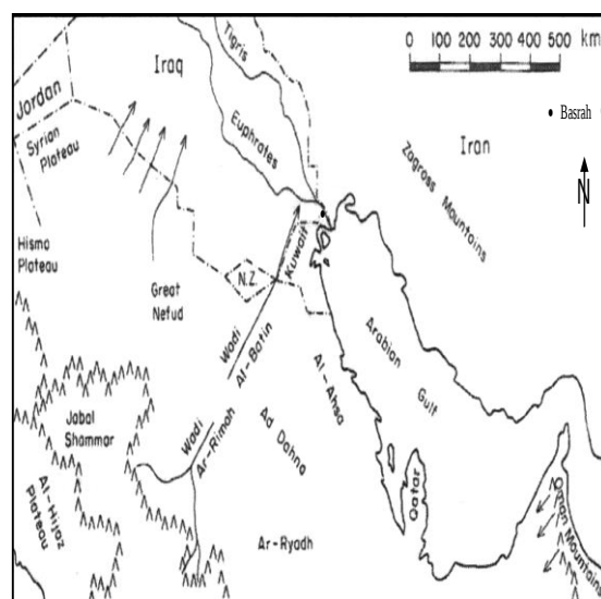
Figure -1: Map showing physiographic province of the northern part of Arabian Peninsula after khalf and Al-Hashash (1983).
