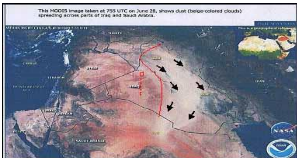
Fig.-4B: Satellite image of Arabian Gulf during a dust storm (NASA, NOAA, 2009)
