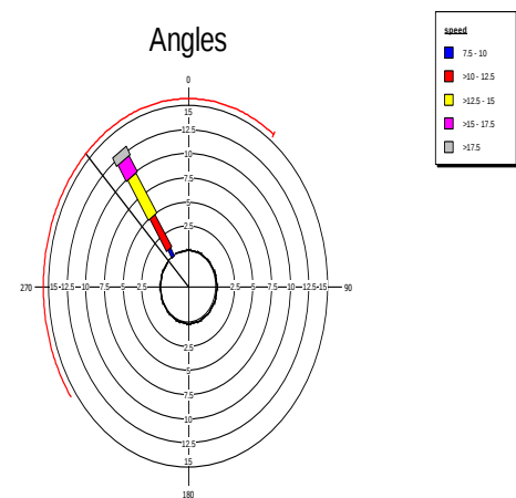
Fig.-3: Wind rose in Iraq based on Al-Khait,( 2002 ) meteorological data
