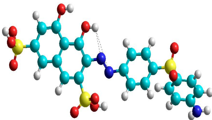
Figure 4. Semi-empirical AM1 calculated optimized structure of configuration of azo dye with intramolecular hydrogen bonding (II) of the possible
