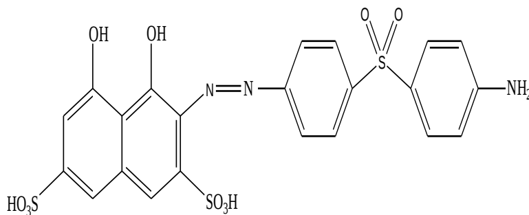
Scheme1. chemical structure of the (4,5-dihydroxy-3-((4-aminodiphenylsulfone)phenyl)diazenyl)naphthalene-2,7-disulfonic acid
