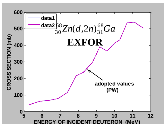
(7): The adopted cross section of the ^{68}_{30}\text{Zn} target t (present work) compared with EXFOR Library. Data 1:Ref. No.[4]; Data 2: (PW).
