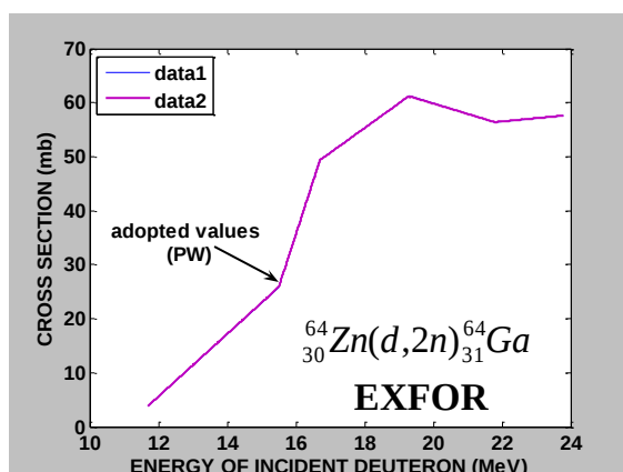
Figure (3): The adopted cross section of the ^{64}_{30}\text{Zn} target element (present work) compared with EXFOR Library. Data 1:Ref. No.[2]; Data 2: (PW).
