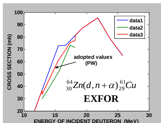
Figure (2): The adopted cross section of the ^{64}_{30}\text{Zn} target element (present work) compared with EXFOR Library. Data 1:Ref. No.[2]; Data 2:Ref. No.[1]; Data 3: (PW).
