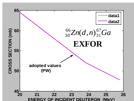
Figure (5): The adopted cross section of the ^{66}_{30}\text{Zn} target element (present work) compared with EXFOR Library. Data 1:Ref. No.[2]; Data 2: (PW).
