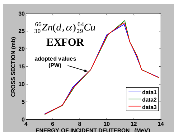
Figure (4): The adopted cross section of the ^{66}_{30}\text{Zn} target element (present work) compared with EXFOR Library. Data 1:Ref. No.[3]; Data 2:Ref. No.[4]; Data 3: (PW).
