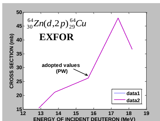
Figure (1): The adopted cross section of the ^{64}_{30}\text{Zn} target element (present work) compared with EXFOR Library. Data 1:Ref. No.[1]; Data 2: (PW).
