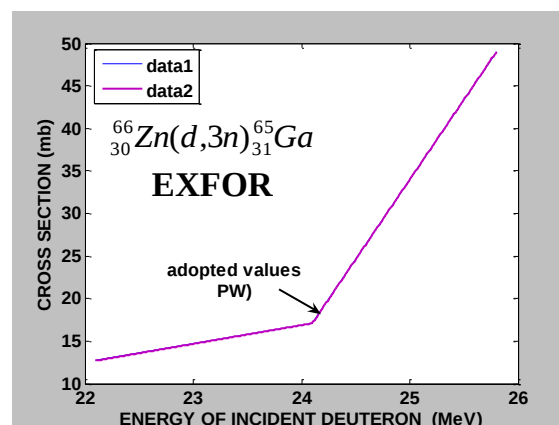
Figure (6): The adopted cross section of the ^{66}_{30}\text{Zn} target element (present work) compared with EXFOR Library. Data 1:Ref. No.[2]; Data 2: (PW).
