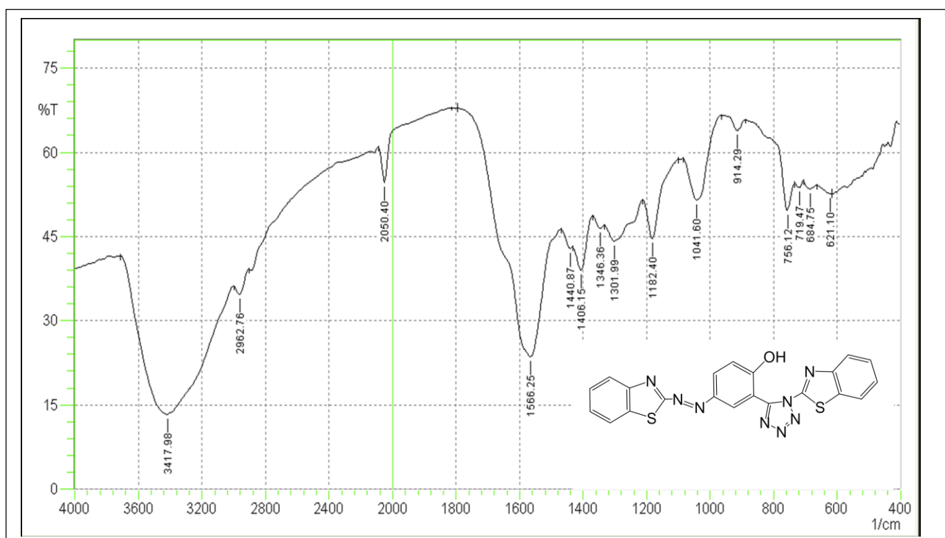
Fig-6: FT-IR spectrum of compound 4
