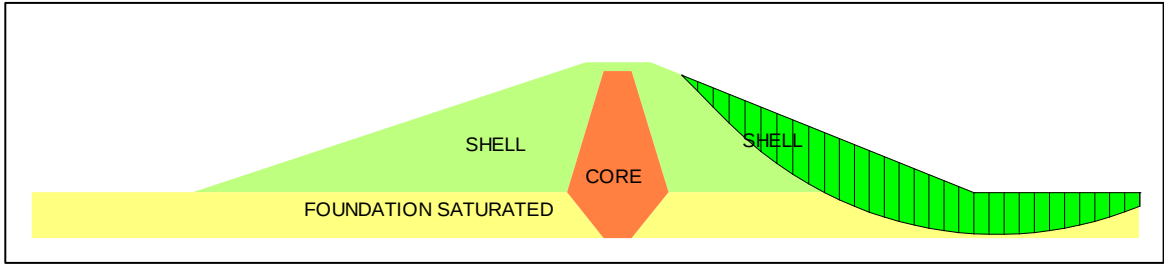
Figure (9): The factor of safety for earth dam.
