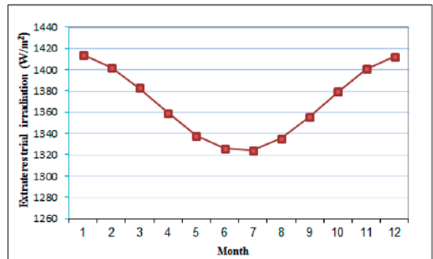
Figure (6): The relation between sun irradiance extraterrestrial and month of the year.
