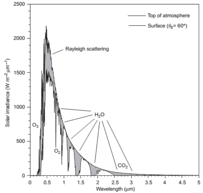
Figure(2): The Rayleigh scattering[M. Santamourois].
