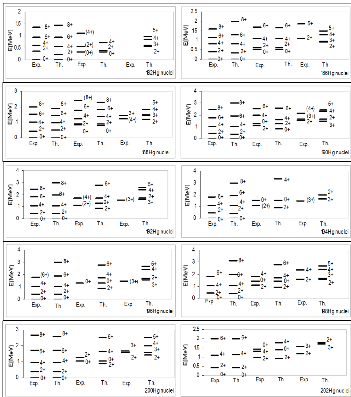
Fig. (2): A comparison between theoretical values of energy levels and the corresponding experimental one for ^{182-202}\text{Hg} .
