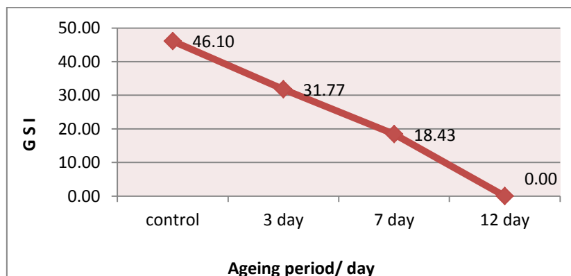
Fig (3) Effect of accelerated ageing conditions on germination speed index (GSI) for snake cucumber seeds.L.S.D 0.05 = 2.171.
