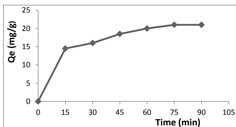
Fig.3 Effect of contact time on adsorption ABZ dye by ZnO surface
