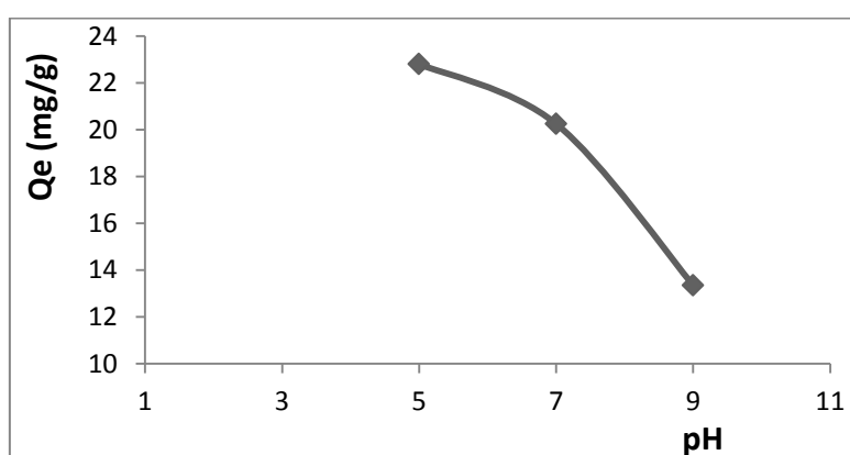
Fig.6 Effect of pH for adsorption ABZ by ZnO surface
