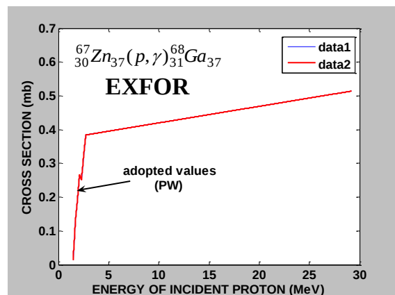
Figure (6): The adopted cross section of the ^{67}_{30}\text{Zn}_{37}(p, \gamma)^{68}_{31}\text{Ga}_{37} target element (present work) compared with EXFOR Library. Data 1:Ref. No.[9]; Data 2: (PW).
