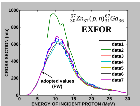
Figure (5): The adopted cross section of the ^{67}_{30}\text{Zn}_{37}(p, n)^{67}_{31}\text{Ga}_{36} target element (present work) compared with EXFOR Library. Data 1:Ref. No.[15]; Data 2:Ref. No.[12]; Data 3:Ref. No.[17]; Data 4:Ref. No.[18]; Data 5:Ref. No.[19]; Data 6:Ref. No.[19]; Data 7: (PW)
