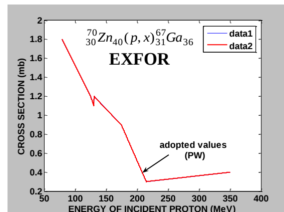
Figure (12): The adopted cross section of the ^{70}_{30}\text{Zn}_{40}(p,x)^{67}_{31}\text{Ga}_{36} target element (present work) compared with EXFOR Library. Data 1:Ref. No.[31]; Data 2: (PW).
