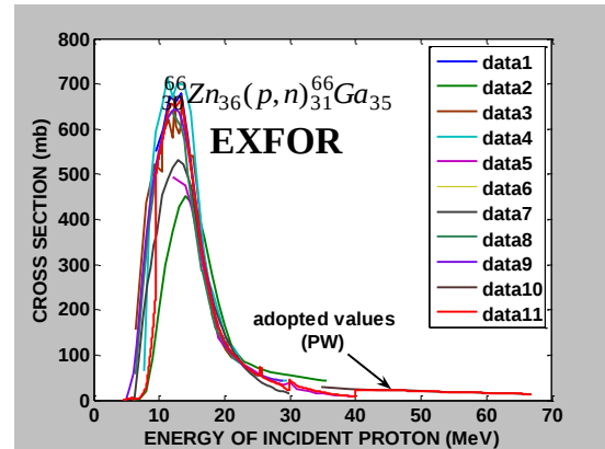
Figure (2): The adopted cross section of the ^{66}_{30}\text{Zn}_{36}(p, n)^{66}_{31}\text{Ga}_{35} target element (present work) compared with EXFOR Library. Data 1:Ref. No.[13]; Data 2:Ref. No.[14]; Data 3:Ref. No.[15]; Data 4:Ref. No.[12]; Data 5:Ref. No.[16]; Data 6:Ref. No.[17]; Data 7:Ref. No.[18]; Data 8:Ref. No.[19]; Data 9:Ref. No.[19]; Data 10:Ref. No.[20]; Data 11: (PW).
