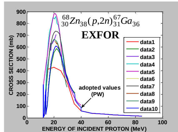
Figure (8): The adopted cross section of the ^{68}_{30}\text{Zn}_{38}(p,2n)^{67}_{31}\text{Ga}_{36} target element (present work) compared with EXFOR Library. Data 1:Ref. No.[21]; Data 2:Ref. No.[14]; Data 3:Ref. No.[22]; Data 4:Ref. No.[12]; Data 5:Ref. No.[16]; Data 6:Ref. No.[17]; Data 7:Ref. No.[18]; Data 8:Ref. No.[19]; Data 9:Ref. No.[19]; Data 10: (PW).
