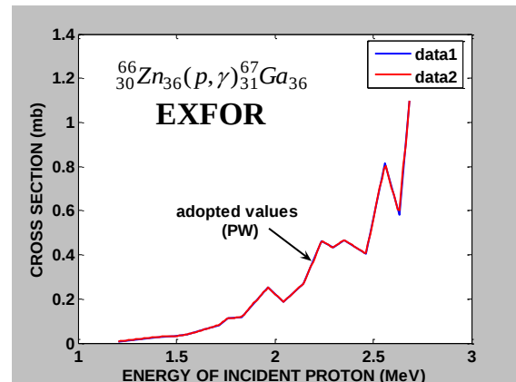
Figure (4): The adopted cross section of the ^{66}_{30}\text{Zn}_{36}(p, \gamma)^{67}_{31}\text{Ga}_{36} target element (present work) compared with EXFOR Library. Data 1:Ref. No.[10]; Data 2: (PW).
