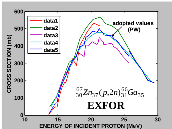
Figure (7): The adopted cross section of the ^{67}_{30}\text{Zn}_{37}(p,2n)^{66}_{31}\text{Ga}_{35} target element (present work) compared with EXFOR Library. Data 1:Ref. No.[15]; Data 2:Ref. No.[12]; Data 3:Ref. No.[17]; Data 4:Ref. No.[19]; Data 5: (PW).
