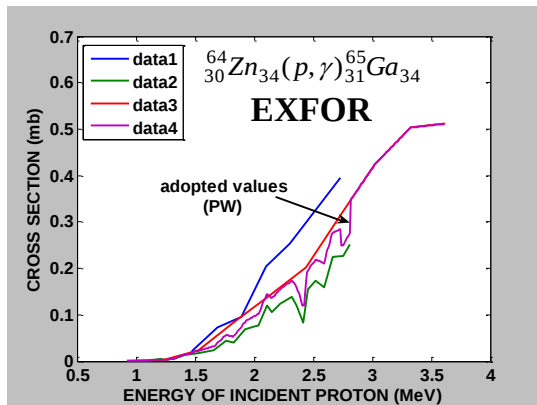
Figure (1): The adopted cross section of the ^{64}_{30}\text{Zn}_{34}(p, \gamma)^{65}_{31}\text{Ga}_{34} target element (present work) compared with EXFOR Library. Data 1:Ref. No.[9]; Data 2:Ref. No.[10]; Data 3:Ref.
