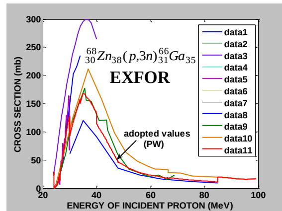
Figure (10): The adopted cross section of the ^{68}_{30}\text{Zn}_{38}(p,3n)^{66}_{31}\text{Ga}_{35} target element (present work) compared with EXFOR Library. Data 1:Ref. No.[21]; Data 2:Ref. No.[12]; Data 3:Ref. No.[16]; Data 4:Ref. No.[17]; Data 5:Ref. No.[18]; Data 6:Ref. No.[19]; Data 7:Ref. No.[19]; Data 8:Ref. No.[28]; Data 9:Ref. No.[29]; Data 10: Ref. No. [30]; Data 11: (PW).
