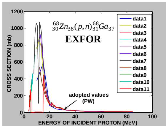
Figure (9): The adopted cross section of the ^{68}_{30}\text{Zn}_{38}(p,n)^{68}_{31}\text{Ga}_{37} target element (present work) compared with EXFOR Library. Data 1:Ref. No.[21]; Data 2:Ref. No.[13]; Data 3:Ref. No.[23]; Data 4:Ref. No.[24]; Data 5:Ref. No.[25]; Data 6:Ref. No.[15]; Data 7:Ref. No.[12]; Data 8:Ref. No.[16]; Data 9:Ref. No.[26]; Data 10: Ref. No. [27]; Data 11: (PW).
