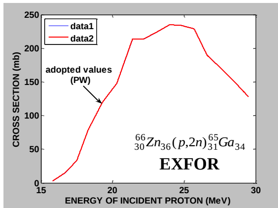
Figure (3): The adopted cross section of the ^{66}_{30}\text{Zn}_{36}(p, 2n)^{65}_{31}\text{Ga}_{34} target element (present work) compared with EXFOR Library. Data 1:Ref. No.[12]; Data 2: (PW).
