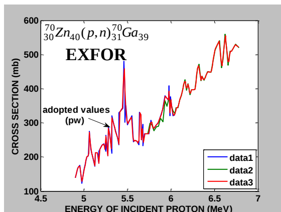
Figure (11): The adopted cross section of the ^{70}_{30}\text{Zn}_{40}(p,n)^{70}_{31}\text{Ga}_{39} target element (present work) compared with EXFOR Library. Data 1:Ref. No.[26]; Data 2: Ref. No.[27]; Data 3: (PW).
