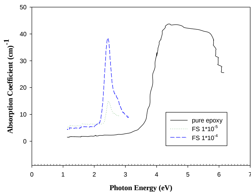
Fig.(5)Optical absorption coefficient vs. photon energy of pure and concentrated epoxy with fluorescein- sodium dye.
