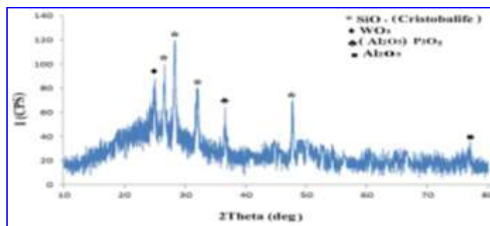
Figure (4) The results of X-ray diffraction analysis of the laser and LED sample on the sample at the same time
