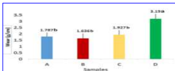
Figure (14): Evaluation of wear between group D with groups A, B, C by Duncan test
