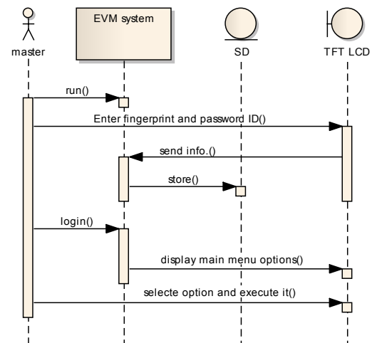
Figure 11: Sequence diagram that describe the operations of master user.
