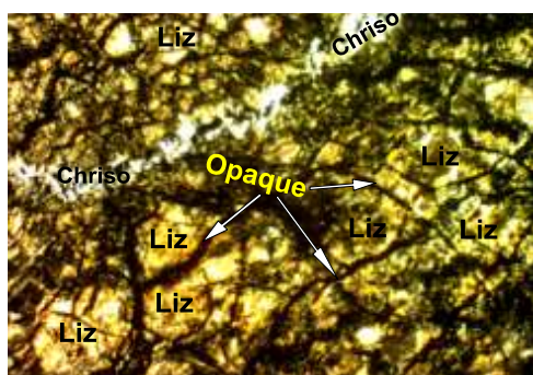
Fig. (12): The lizardite variety after olivine (XN)-(40X) .
