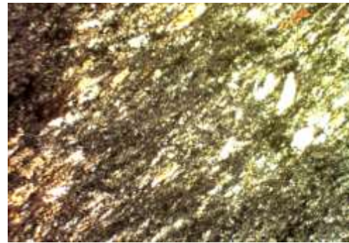
Fig. (3a): Mesh texture which has false Pyroxene crystals appearing in it within fine background of serpentine and this texture is descended from the original rocks
