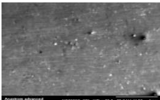
Figure 9: Microscope photograph by (SEM) which shows the structure of Alloy(B) before the oxidation
