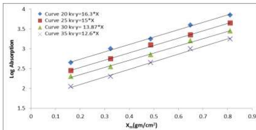
Figure 37 : The relation between Log absorption and equivalent thickness (gm/cm 2 ) for Alloy(B) at 100 °C at (6)h.
