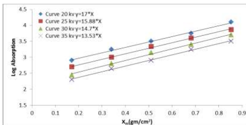
Figure 36 : The relation between Log absorption and equivalent thickness ( \text{gm}/\text{cm}^2 ) for Alloy (A) at 100^\circ\text{C} at (6)h.
