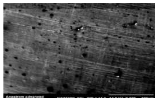
Figure13: Microscope photograph by (SEM) which shows the structure of Alloy(B)after the oxidation(1.5)h
