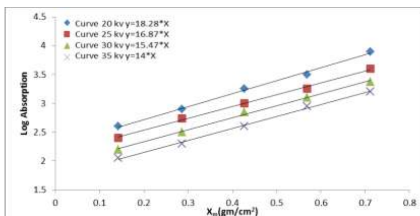
Figure 35 : The relation between Log absorption and equivalent thickness ( \text{gm}/\text{cm}^2 ) for zinc at 100^\circ\text{C} at (6)h.
