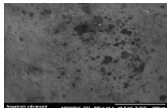
Figure 12: Microscope photograph by (SEM) which shows the structure of Alloy(A)after the oxidation(1.5)h
