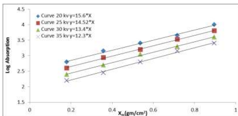
Figure 34 : The relation between Log absorption and equivalent thickness ( \text{gm}/\text{cm}^2 ) for copper at 100^\circ\text{C} at (6)h.
