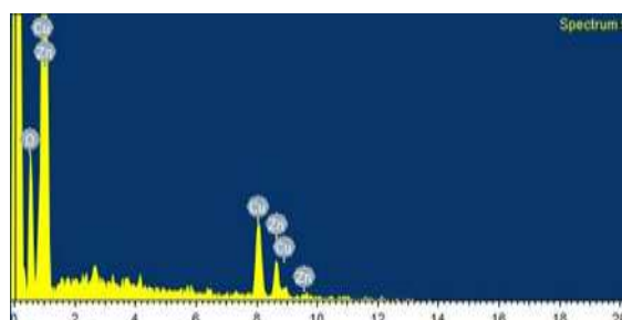
Figure 5 : shows the analysis of the alloy (A) after the oxidation at time (1.5)h.
