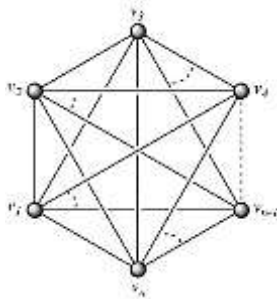
Fig.2. Complete Graph K_n
