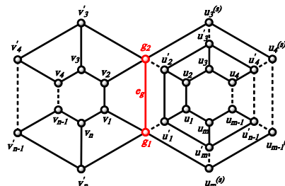
Fig.11. Graph W_{n \times 2}^{m \times s}
