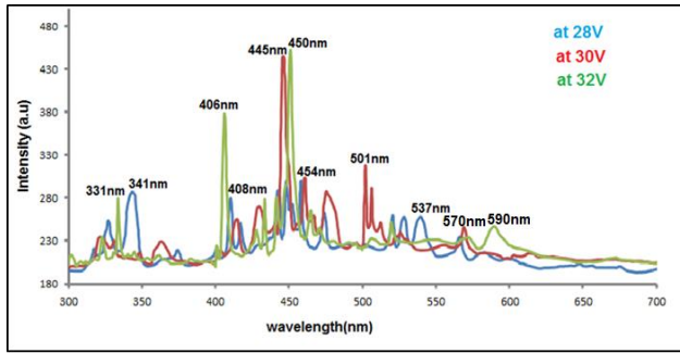
Fig. (4): EL of (TPD:PMMA)/CdS/Alq3 at different voltages
