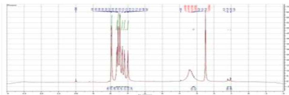
Figure (3) ^1\text{H} NMR for compound (7)
