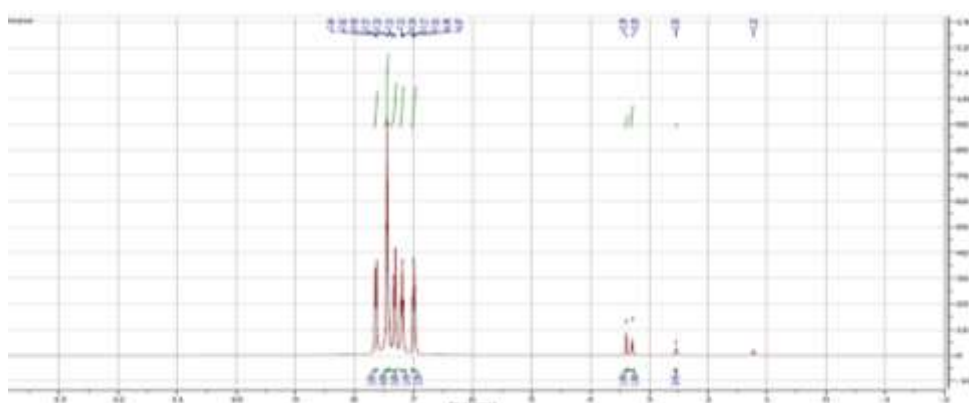
Figure (4) ^1\text{H} NMR for compound (8)
