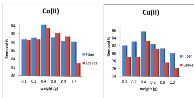
Figure (3) : Effect of the adsorbent weight on rate of Co(II) and Cu(II) removal for the fiber and leaves surfaces at 25 \pm 2 °C, pH 6.5 and contact time 35 min.
