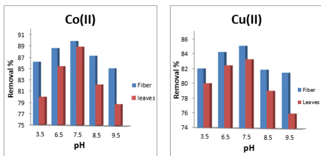
Figure (1) : Effect of pH on rate of Co(II) and Cu(II) removal for the fiber and leaves surfaces at 25 \pm 2 °C.
