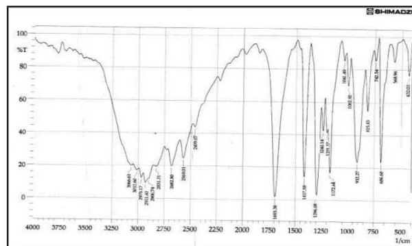
Figure (6): Spectrum FTIR for activated carbon of palm fiber sample.
