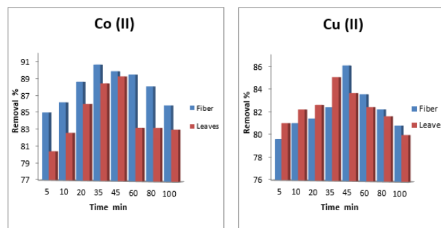
Figure(2): Effect of contact time on rate of Co(II) and Cu(II) removal by fiber and leaves of palm at 25 \pm 2 °C, 0.4 g and pH 6.5.
