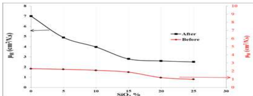
Fig(5) mobility of \text{Zn}_2\text{SiO}_4 before and after annealing
