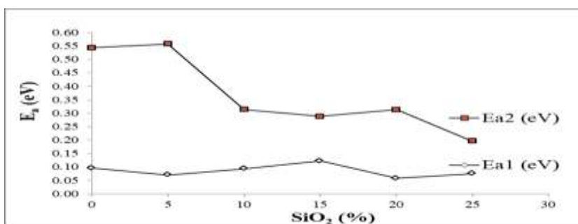
Fig(2) activation energy of Zn_2SiO_4 before annealing
