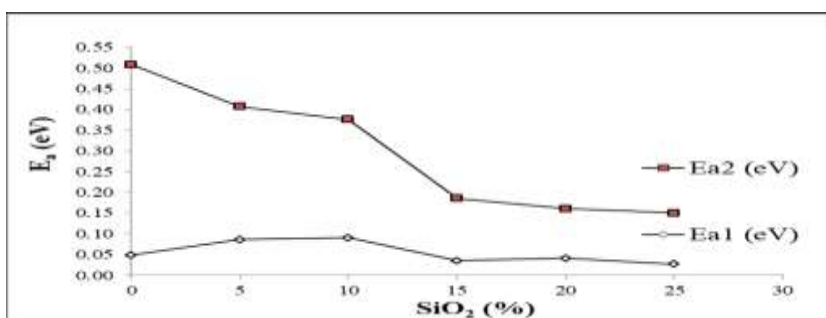
Fig(3) activation energy of Zn_2SiO_4 after annealing
