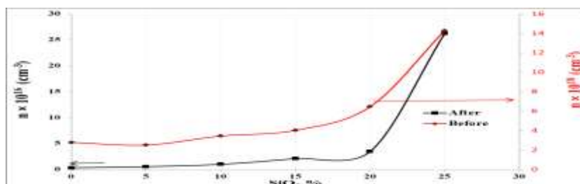
Fig(4) carrier concentration of \text{Zn}_2\text{SiO}_4 before and after annealing
