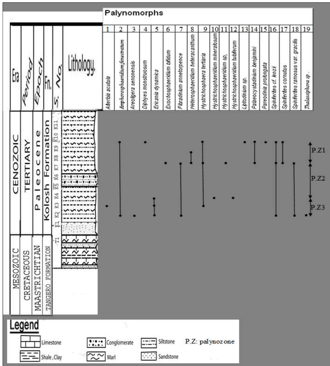
Figure (2): Range chart of selected dinoflagellate cysts species of Kolosh formation in Dokan area Note: the columnar section is not to scale.
