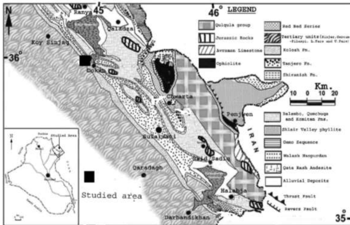
Figure (1): Geological map of the studied area After [13].
