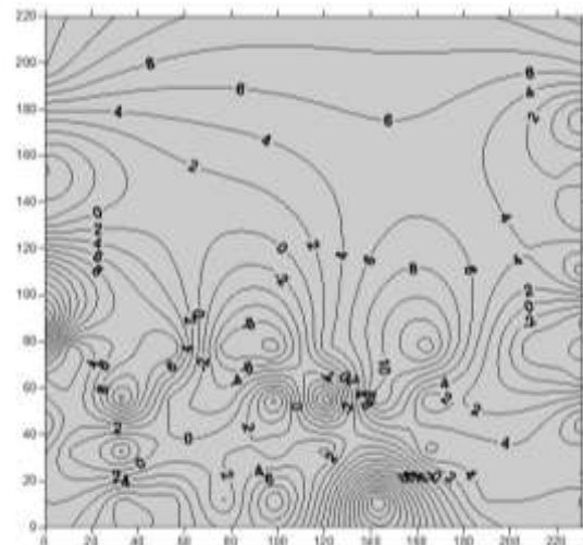
Fig.(4): Observed Self potential contour map.
