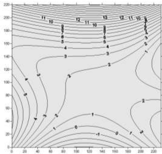
Fig.(5): Regional self potential contour map.
