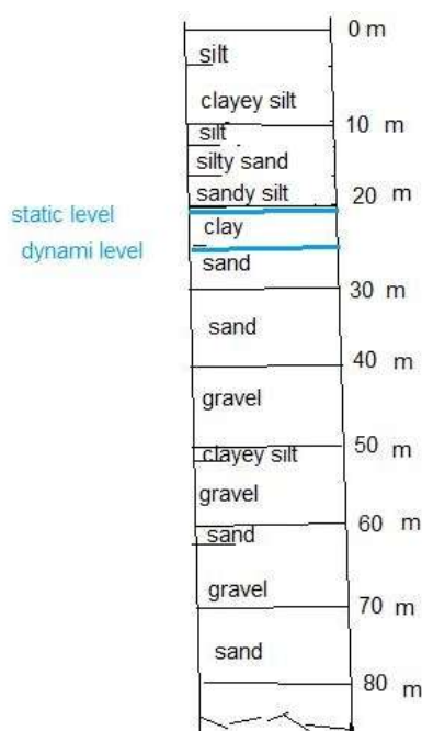
Fig.(8): Borehole geological section and water table.
