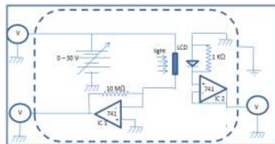
Fig.(3): Electrical measurements Setup
