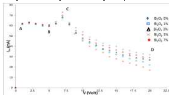
Fig.(6): relationship between voltages and the optical current
