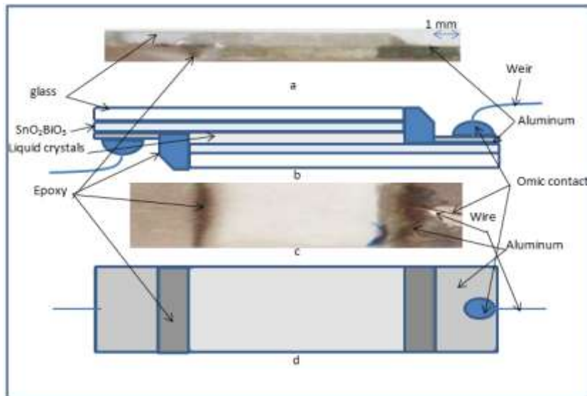
Fig.(1): (a) Vertical image of the cell (b) Vertical chart of the cell (c) horizontal image of the cell (d) horizontal chart of the cell .
