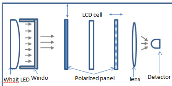
Fig.(2): The system used in the study of optical properties
