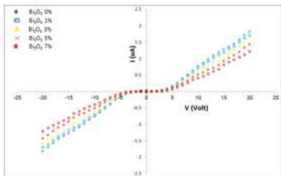
Fig.(4): (I-V) characters of LCD cell in dark
