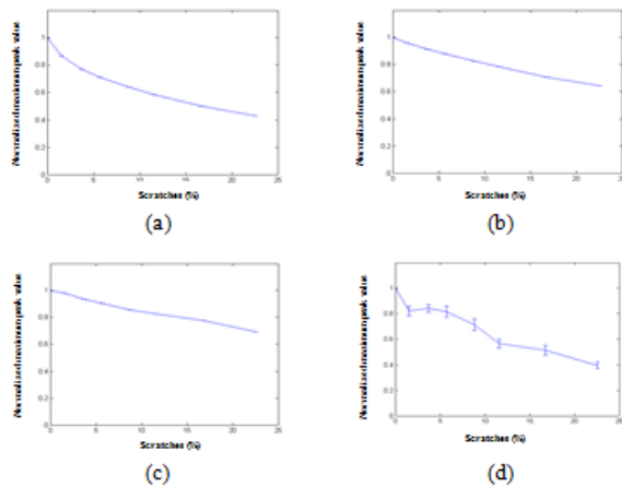
Fig. 10: Normalized maximum peak value of the output correlation as a function of the scratches in percentage for: (a) GCOID tag, (b) GPOID tag based MOEA, (c) BPOID tag based MOEA, (d) and BPOID tag based PC-MOEA tag with N_p = 4000 . The nonlinearity k=0 is applied
