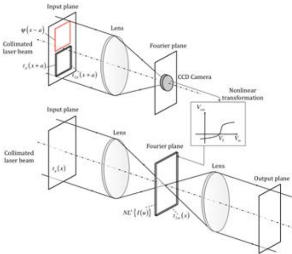
Fig. 1: Architecture of the proposed multifactor optical identity authentication system
